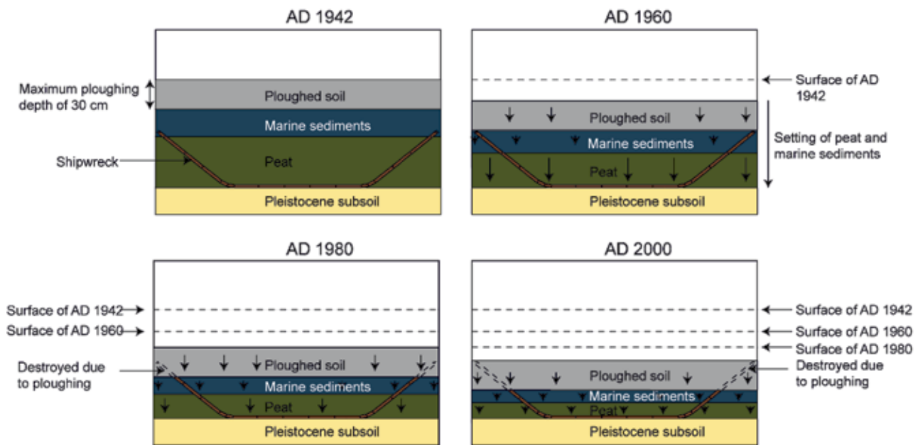
Fig. 13. Simplified model of the effects of soil subsidence and the gradual destruction of shipwrecks (Y.T. van Popta, RUG/GIA).
